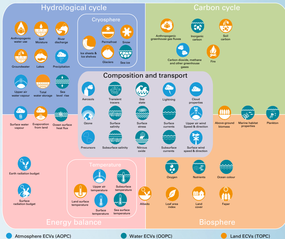
Figure 10. ECVs identified by GCOS and the climate cycles. Many ECVs contribute to understanding several different cycles – this figure only indicates the main links.
